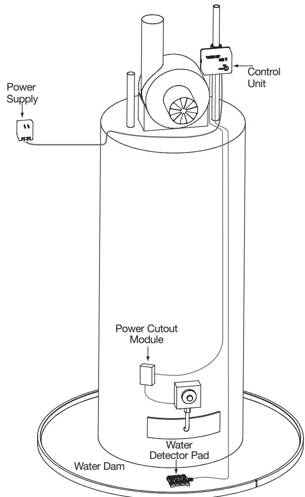
Spark Ignition
